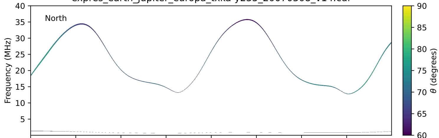
expres_earth_jupiter_europa_txka-y235_20070308_v14.cdf
