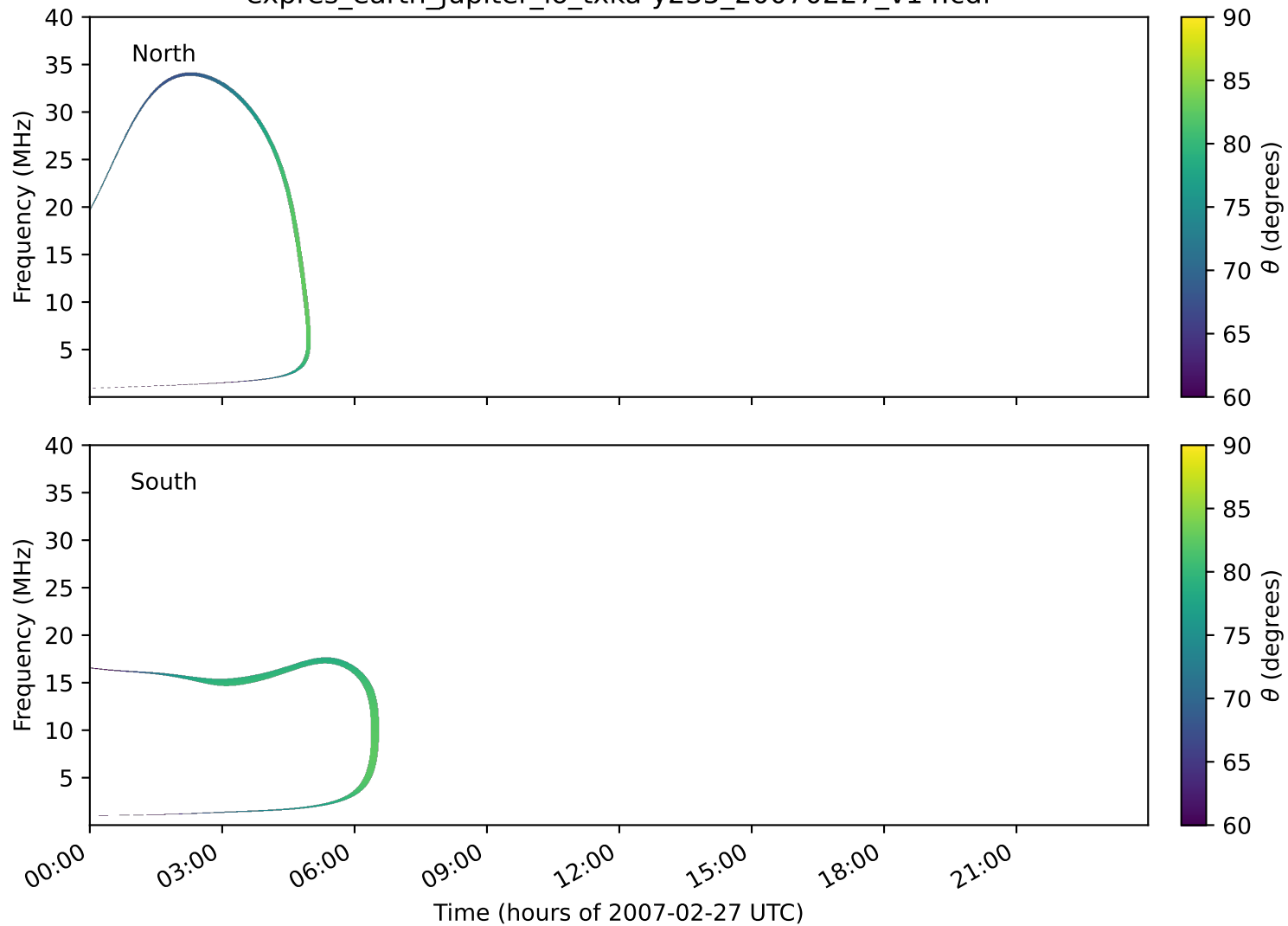
expres_earth_jupiter_io_txka-y235_20070227_v14.cdf
