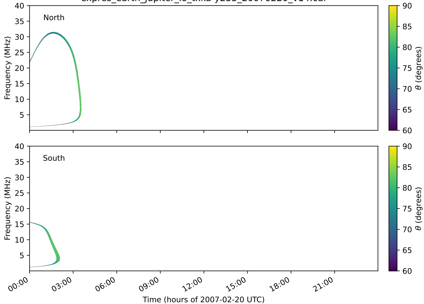
expres_earth_jupiter_io_txka-y235_20070220_v14.cdf
