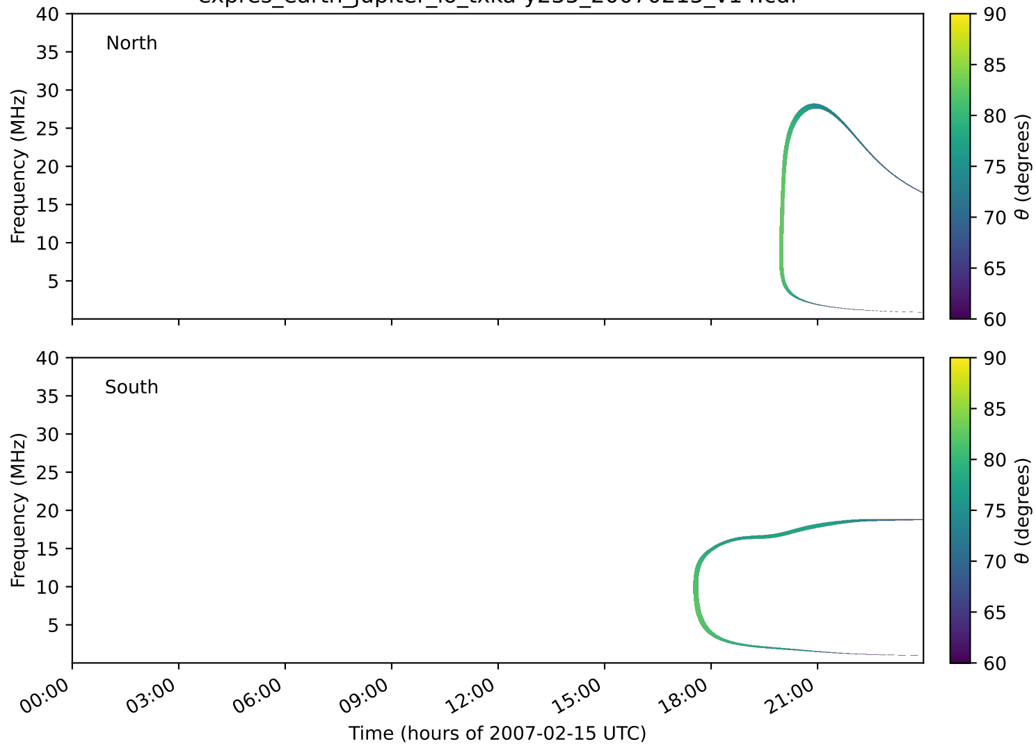
expres_earth_jupiter_io_txka-y235_20070215_v14.cdf
