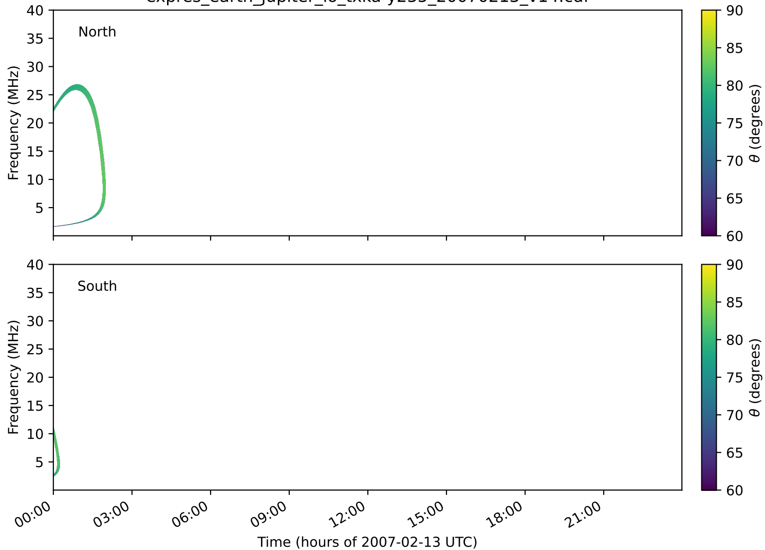
expres_earth_jupiter_io_txka-y235_20070213_v14.cdf
