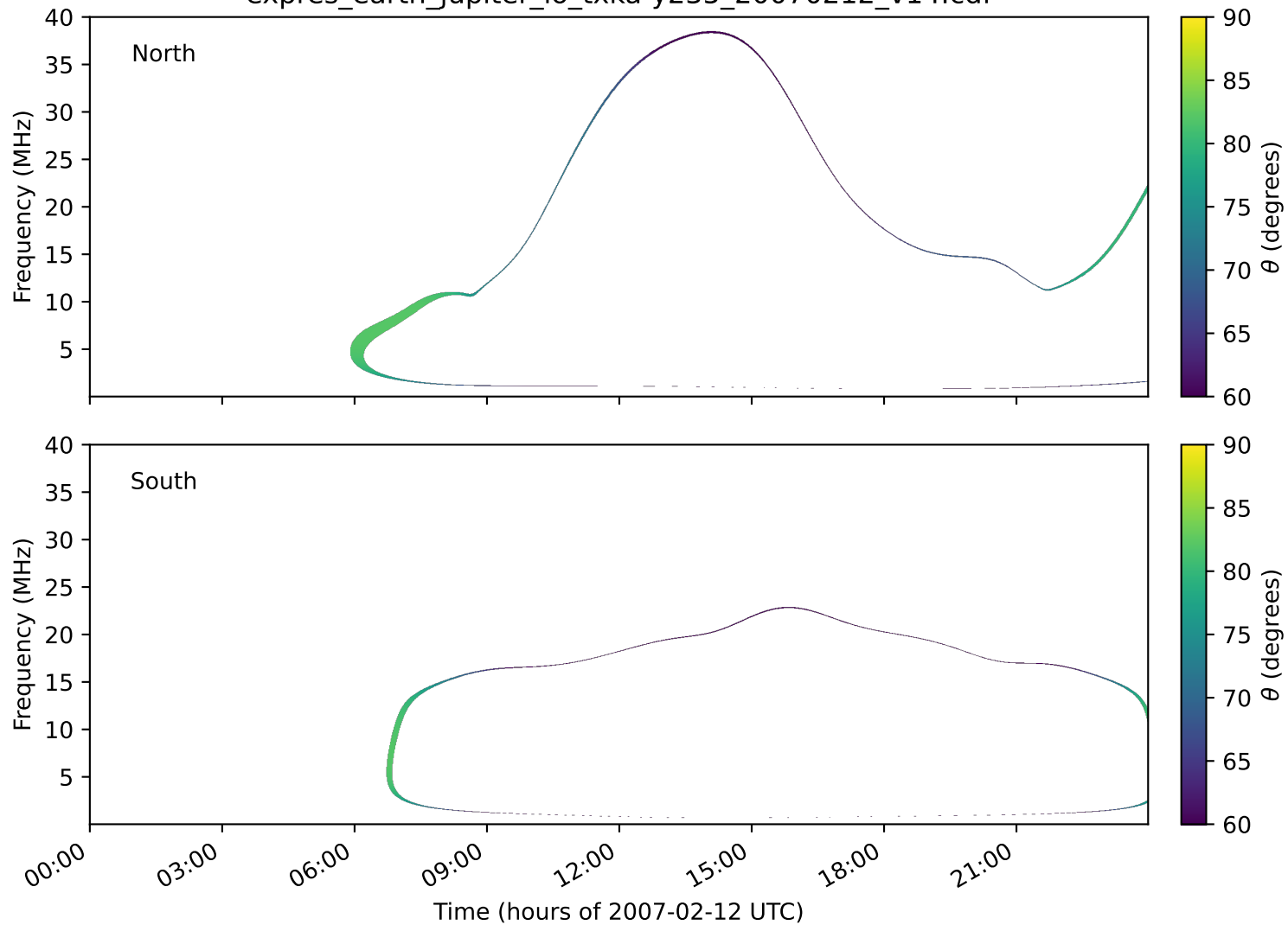
expres_earth_jupiter_io_txka-y235_20070212_v14.cdf
