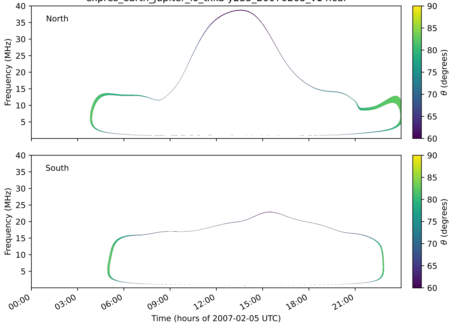
expres_earth_jupiter_io_txka-y235_20070205_v14.cdf
