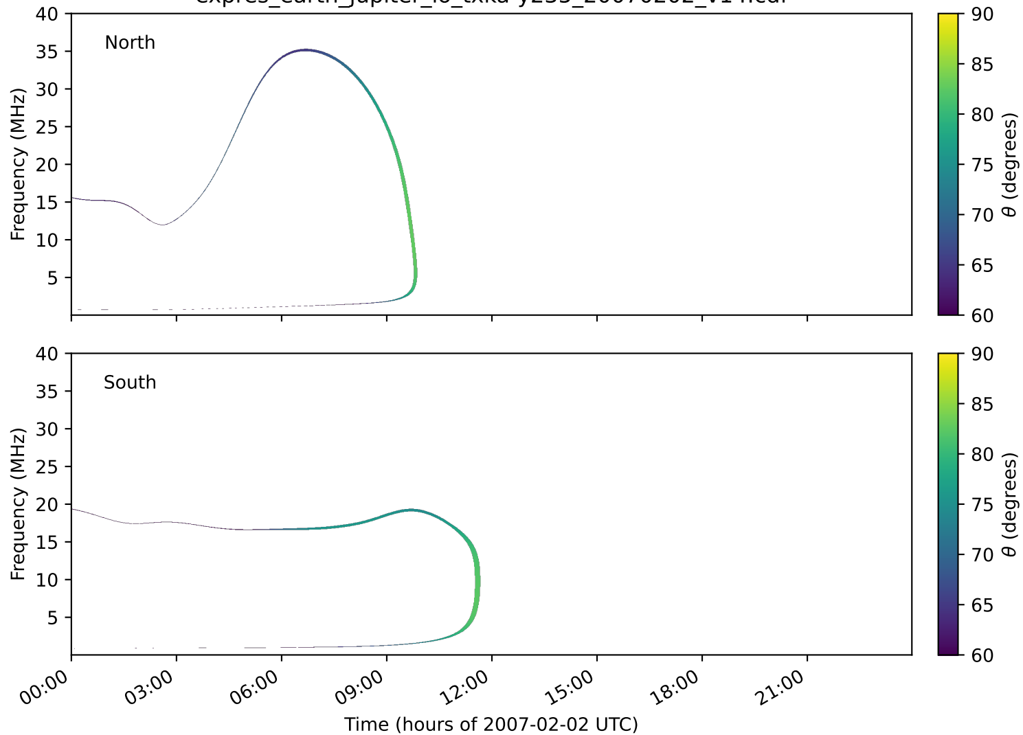
expres_earth_jupiter_io_txka-y235_20070202_v14.cdf
