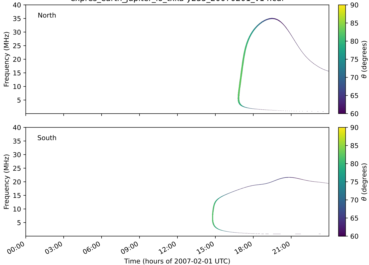
expres_earth_jupiter_io_txka-y235_20070201_v14.cdf
