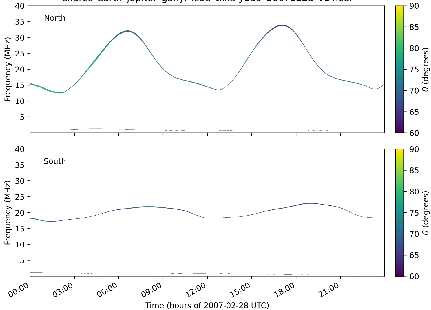
expres_earth_jupiter_ganymede_txka-y235_20070228_v14.cdf
