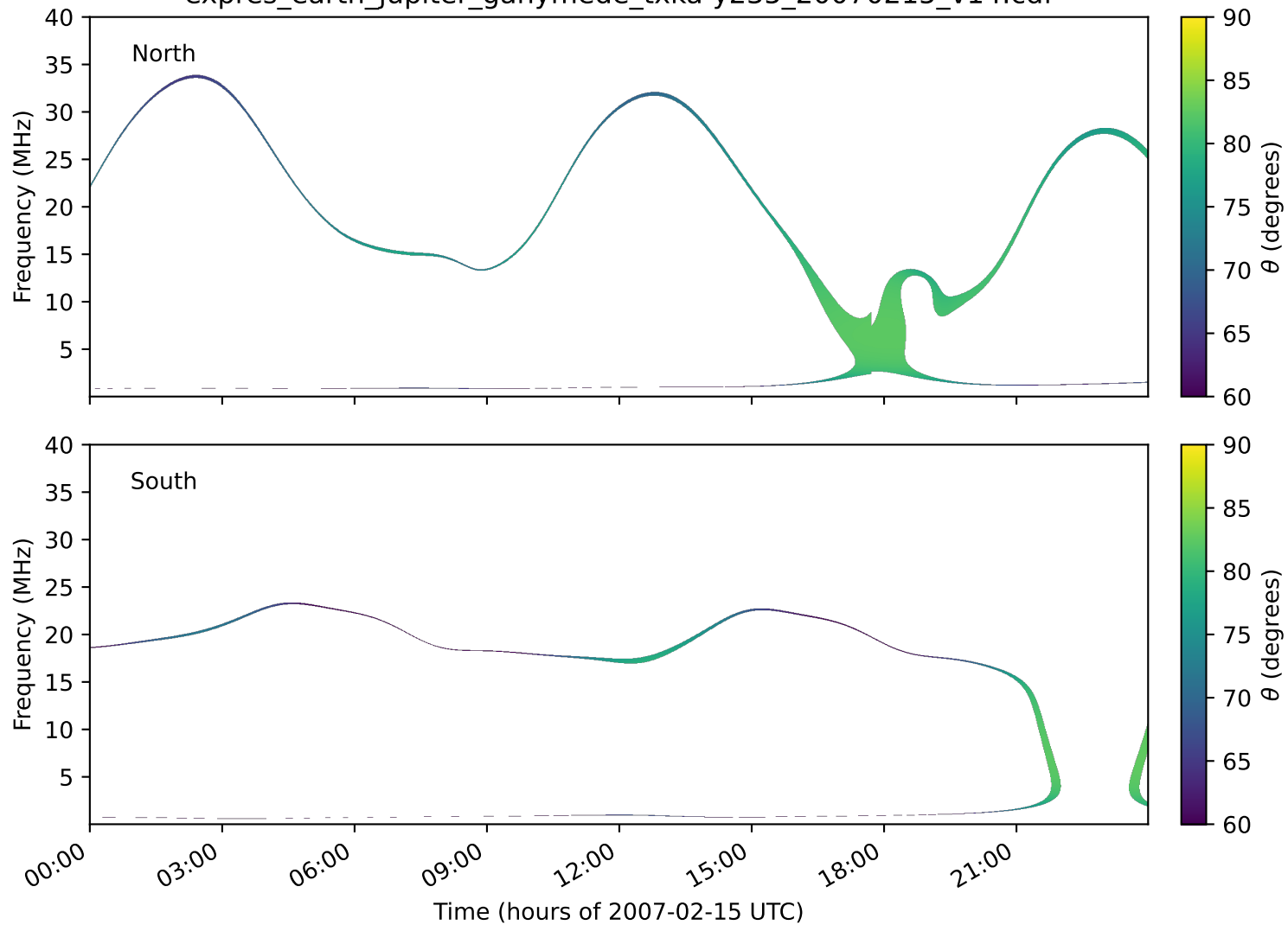
expres_earth_jupiter_ganymede_txka-y235_20070215_v14.cdf
