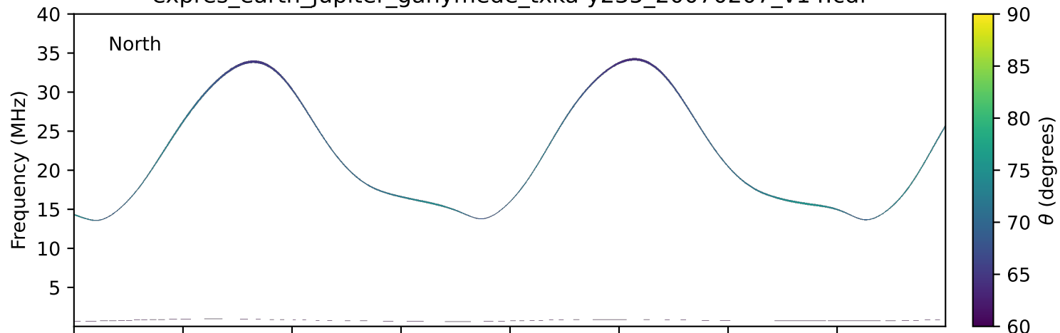
expres_earth_jupiter_ganymede_txka-y235_20070207_v14.cdf
