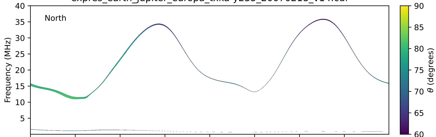
expres_earth_jupiter_europa_txka-y235_20070218_v14.cdf
