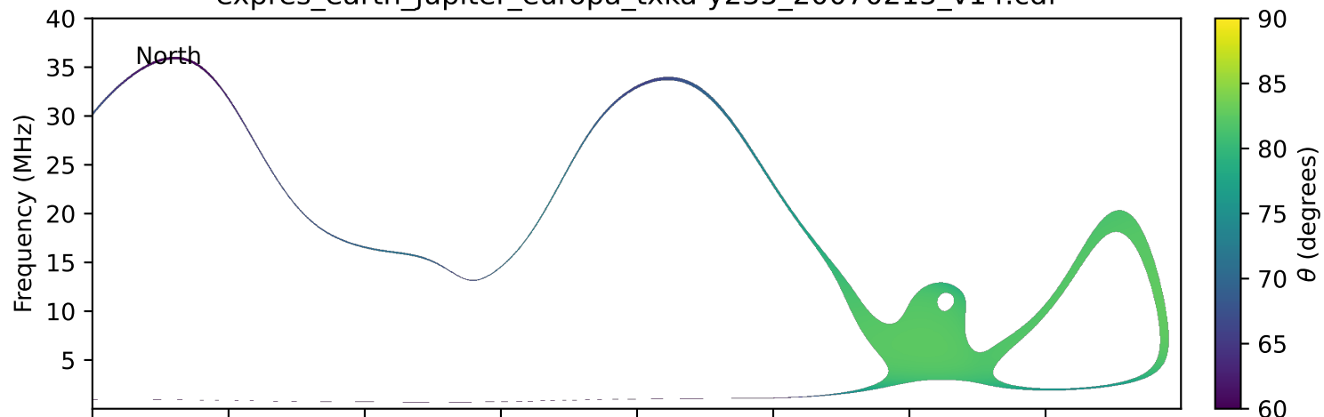
expres_earth_jupiter_europa_txka-y235_20070215_v14.cdf
