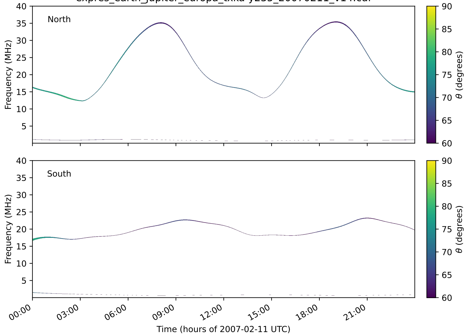
expres_earth_jupiter_europa_txka-y235_20070211_v14.cdf
