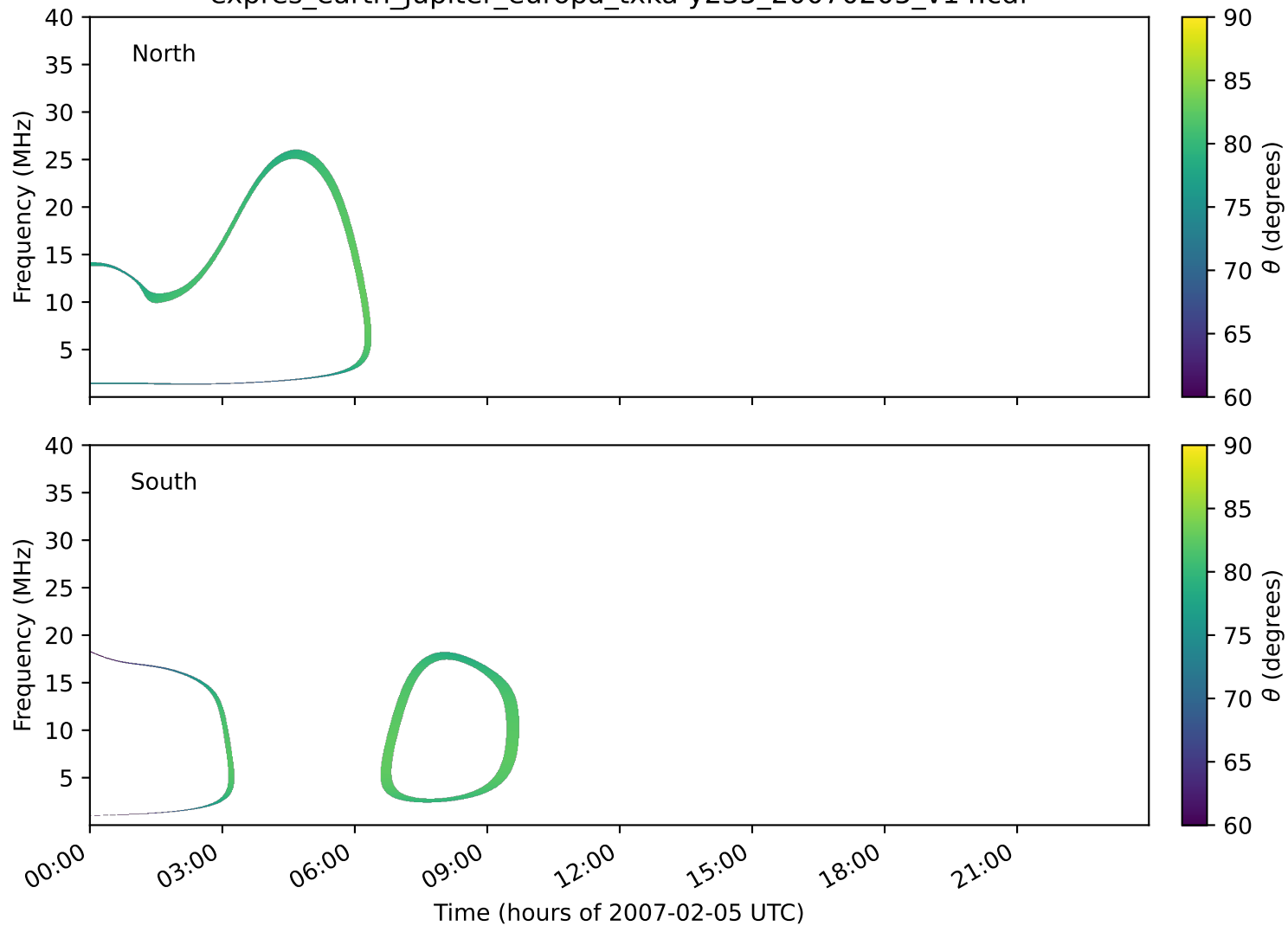
expres_earth_jupiter_europa_txka-y235_20070205_v14.cdf
