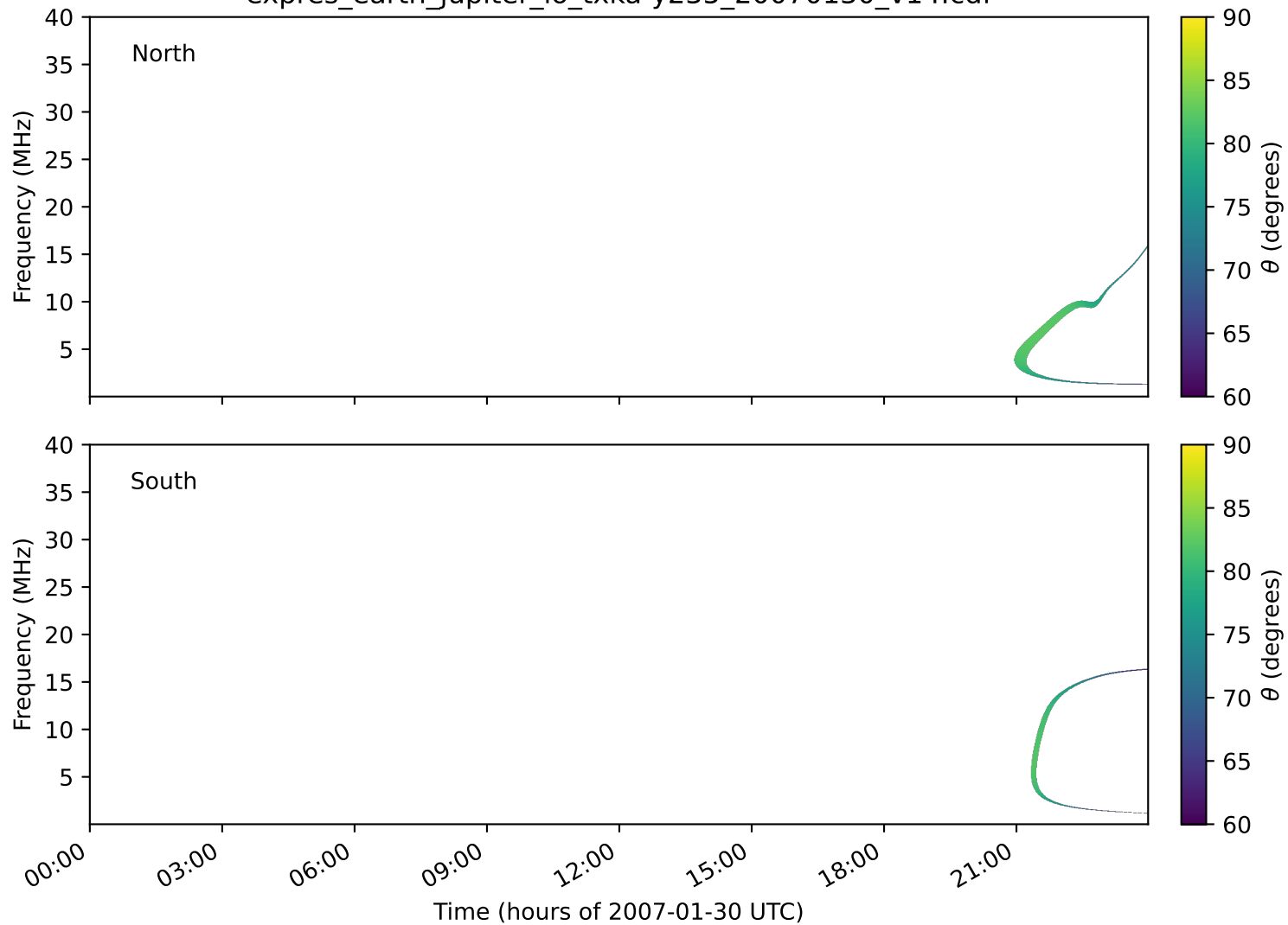
expres_earth_jupiter_io_txka-y235_20070130_v14.cdf
