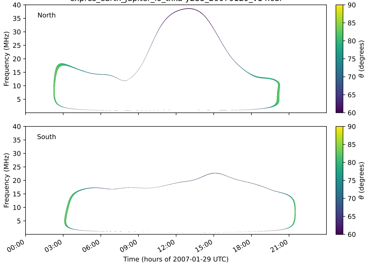
expres_earth_jupiter_io_txka-y235_20070129_v14.cdf
