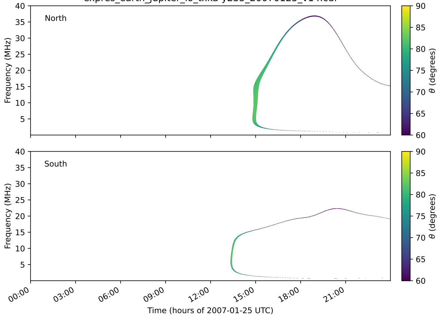
expres_earth_jupiter_io_txka-y235_20070125_v14.cdf
