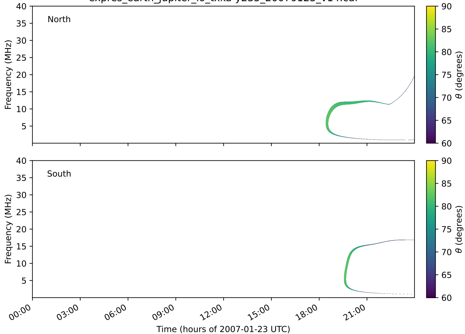
expres_earth_jupiter_io_txka-y235_20070123_v14.cdf
