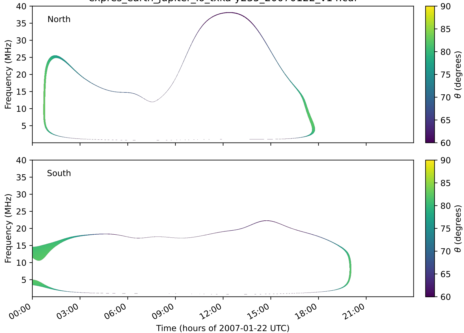
expres_earth_jupiter_io_txka-y235_20070122_v14.cdf
