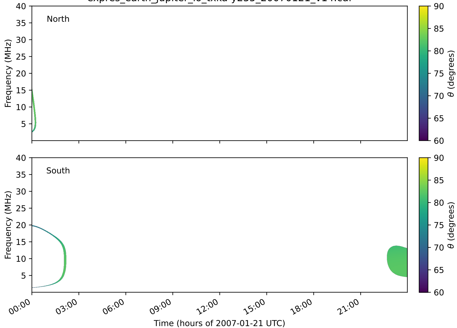
expres_earth_jupiter_io_txka-y235_20070121_v14.cdf
