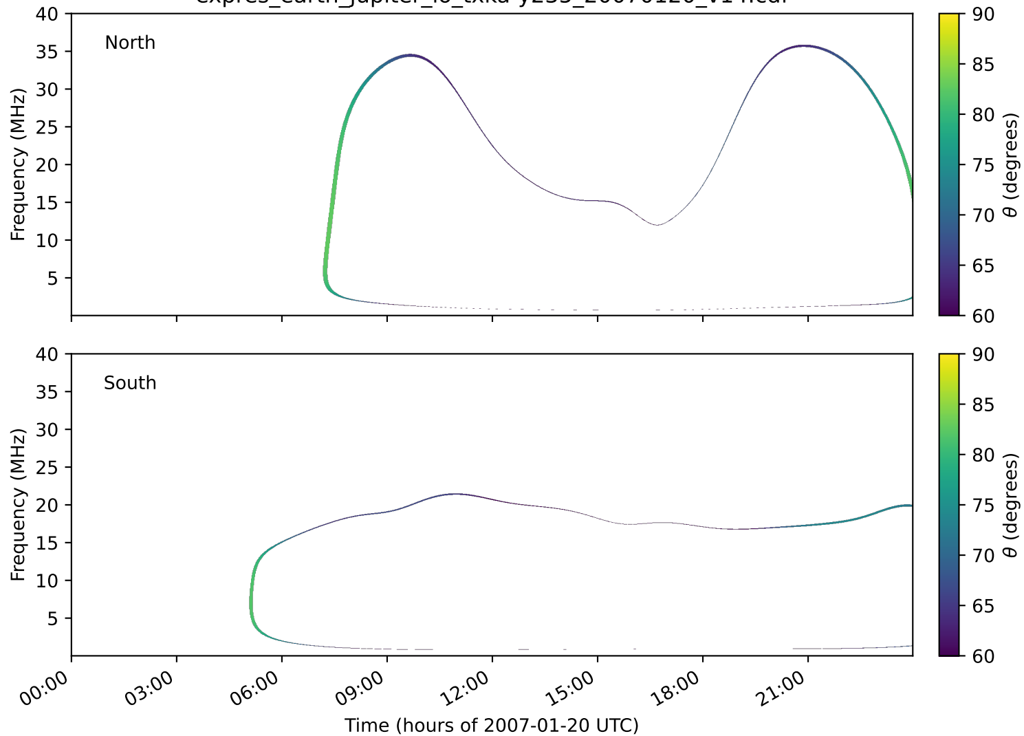
expres_earth_jupiter_io_txka-y235_20070120_v14.cdf
