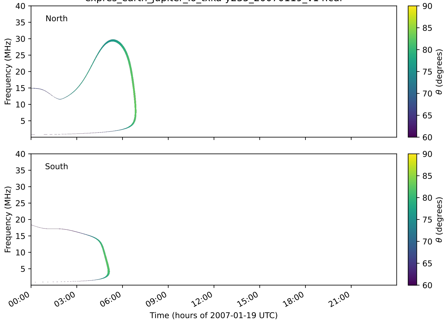
expres_earth_jupiter_io_txka-y235_20070119_v14.cdf
