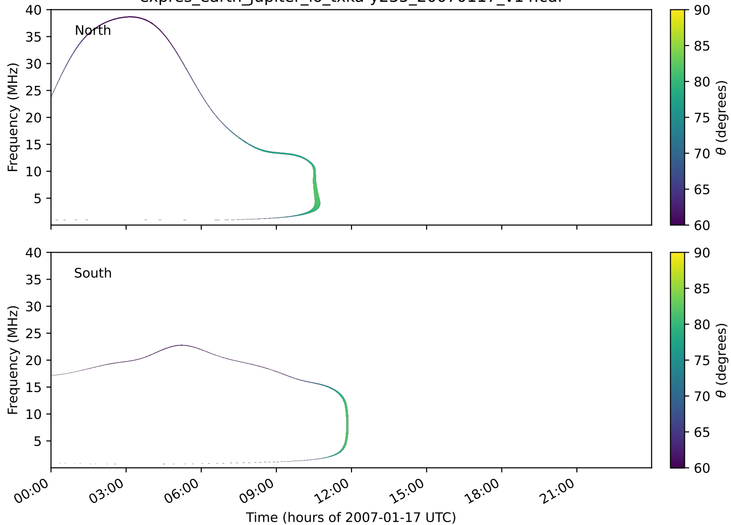
expres_earth_jupiter_io_txka-y235_20070117_v14.cdf
