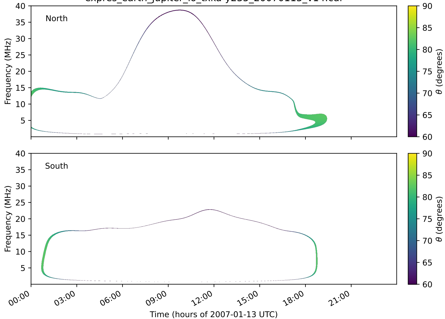
expres_earth_jupiter_io_txka-y235_20070113_v14.cdf
