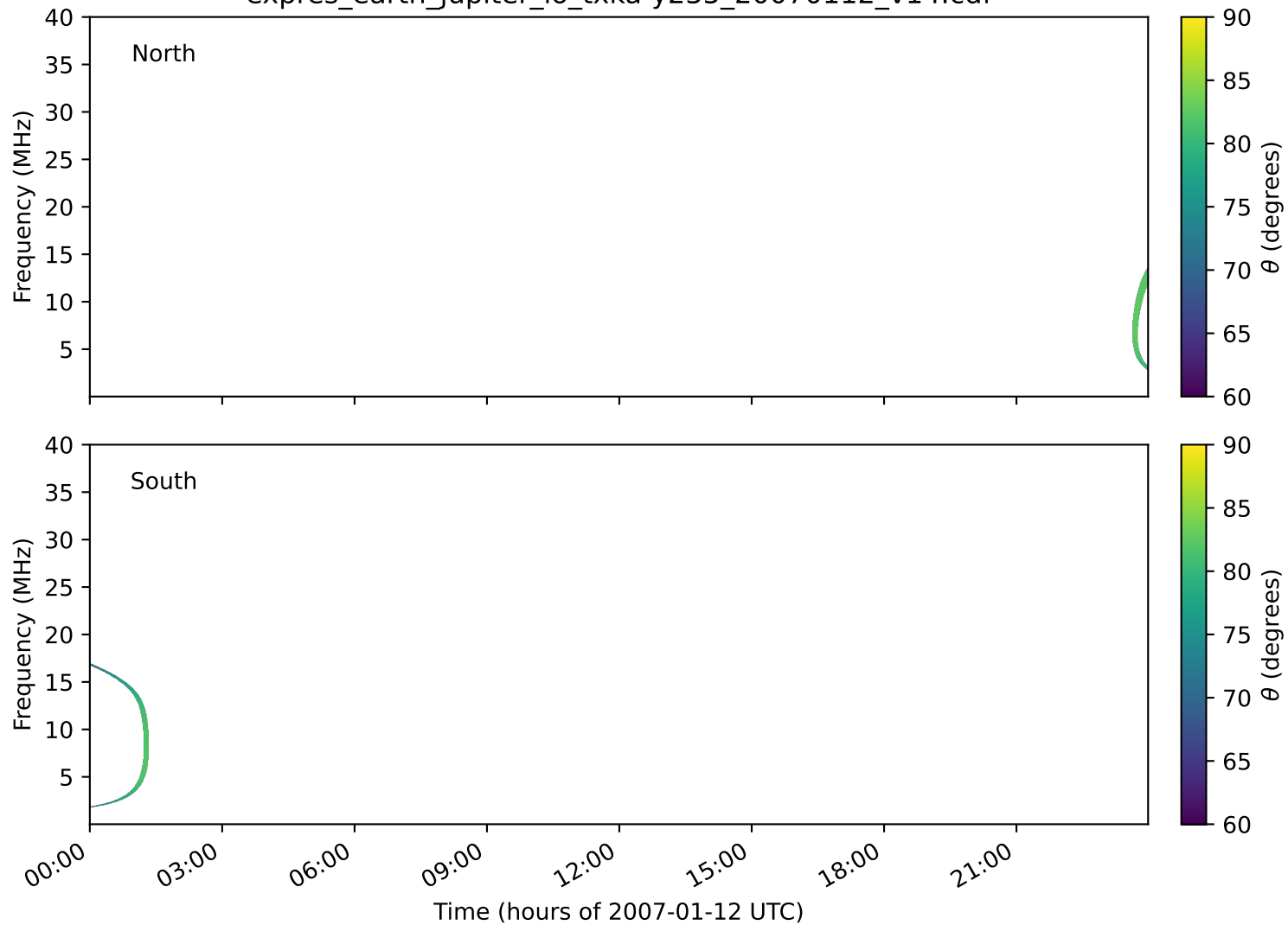
expres_earth_jupiter_io_txka-y235_20070112_v14.cdf
