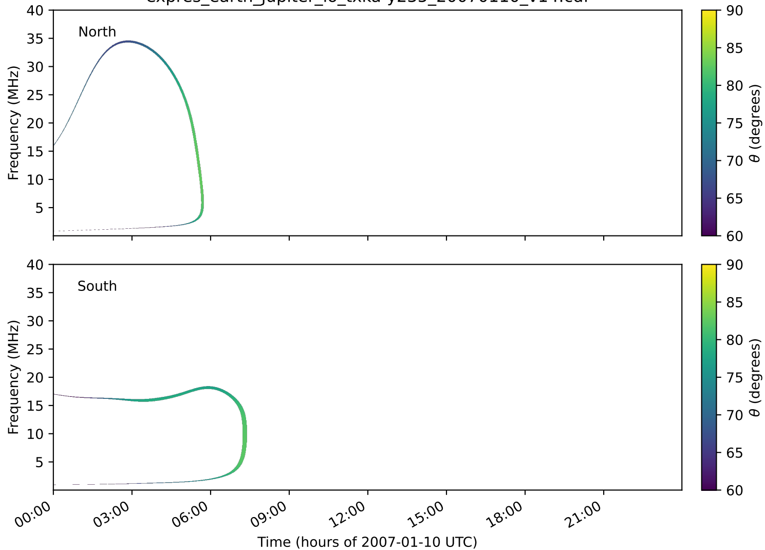
expres_earth_jupiter_io_txka-y235_20070110_v14.cdf
