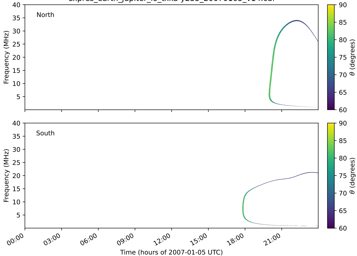
expres_earth_jupiter_io_txka-y235_20070105_v14.cdf
