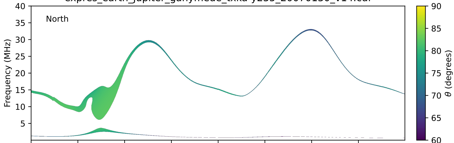
expres_earth_jupiter_ganymede_txka-y235_20070130_v14.cdf
