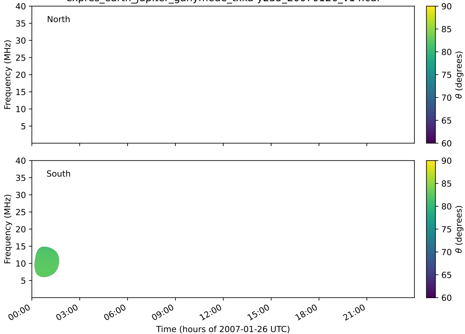
expres_earth_jupiter_ganymede_txka-y235_20070126_v14.cdf
