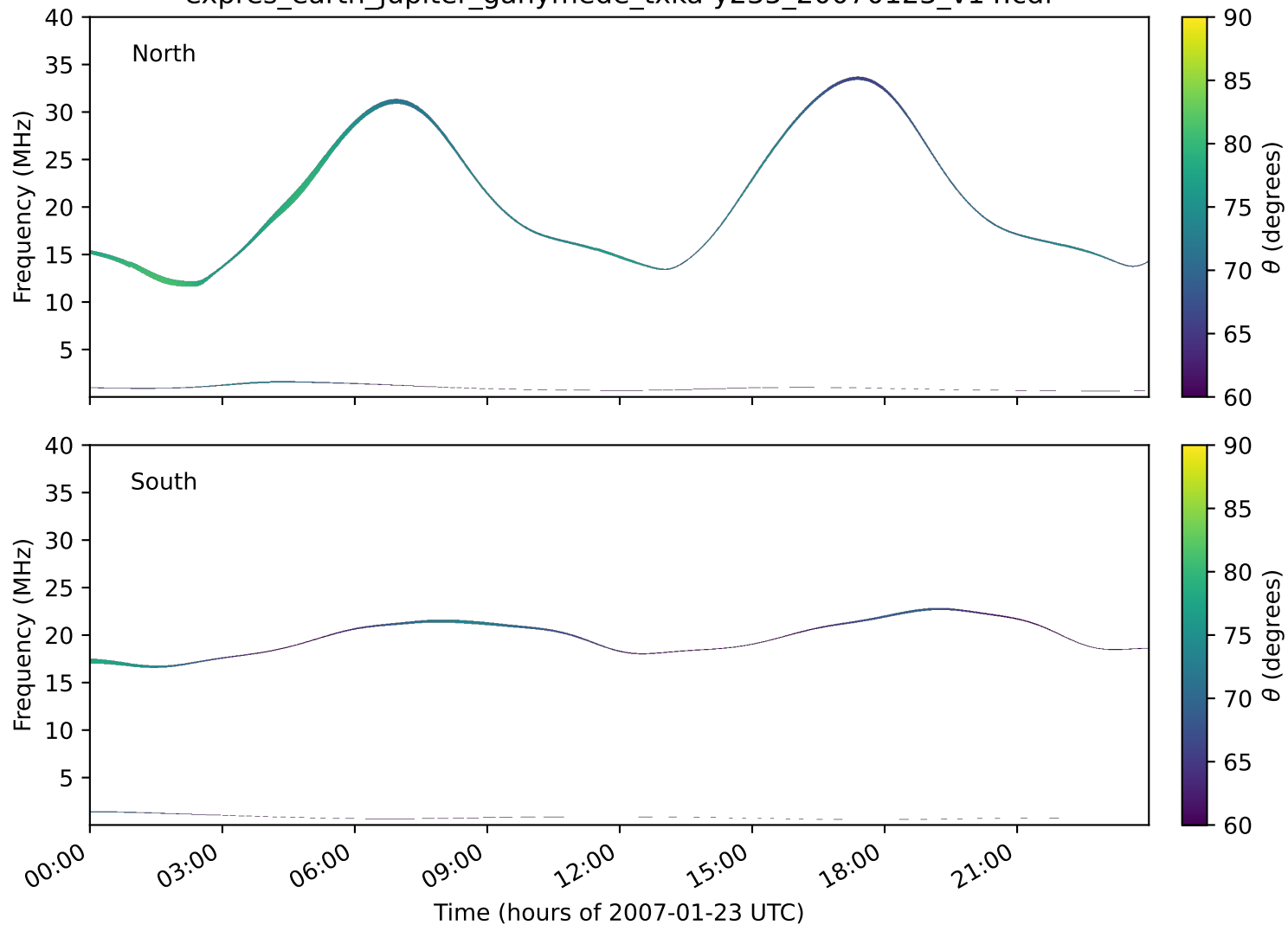
expres_earth_jupiter_ganymede_txka-y235_20070123_v14.cdf
