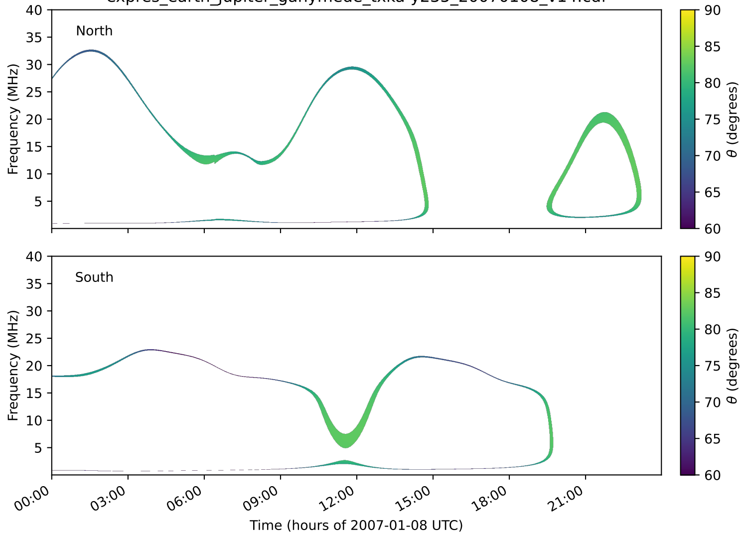
expres_earth_jupiter_ganymede_txka-y235_20070108_v14.cdf
