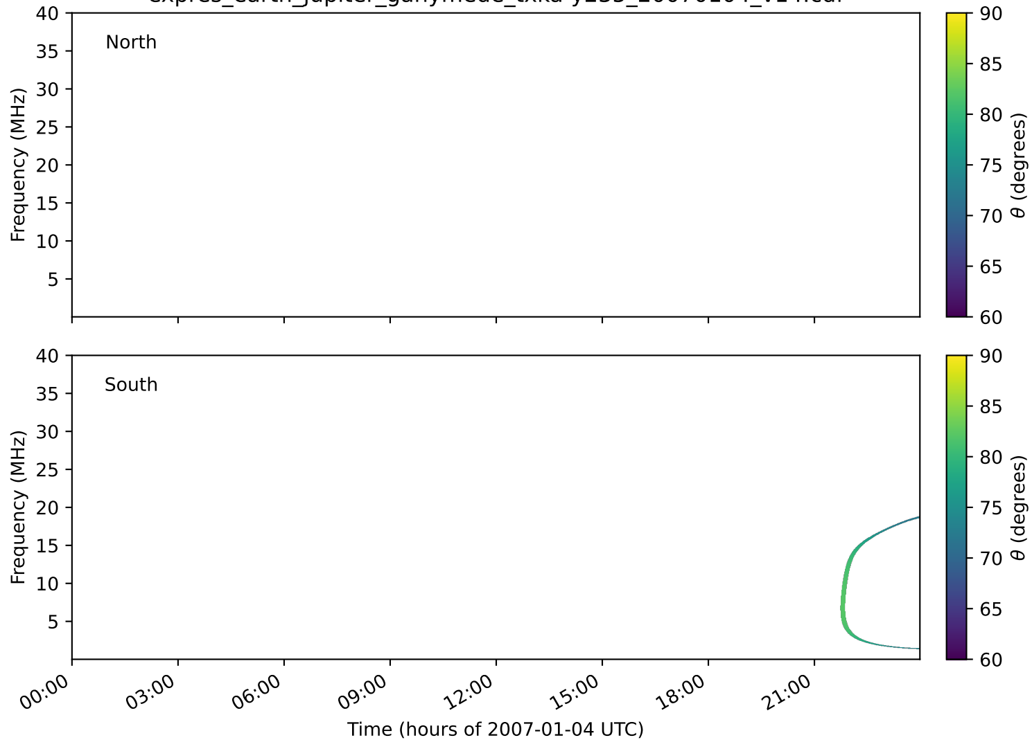
expres_earth_jupiter_ganymede_txka-y235_20070104_v14.cdf
