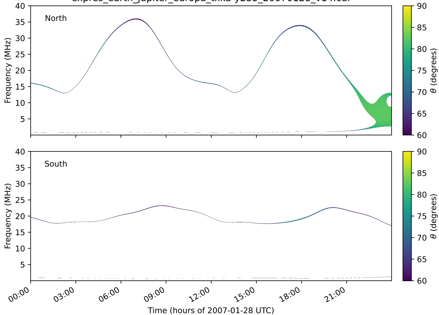
expres_earth_jupiter_europa_txka-y235_20070128_v14.cdf
