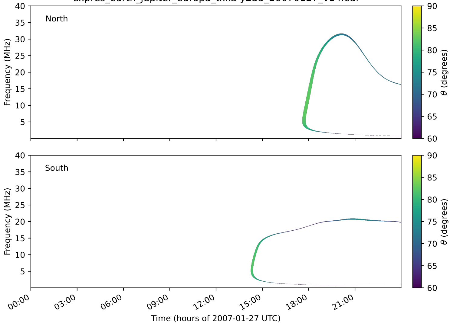
expres_earth_jupiter_europa_txka-y235_20070127_v14.cdf
