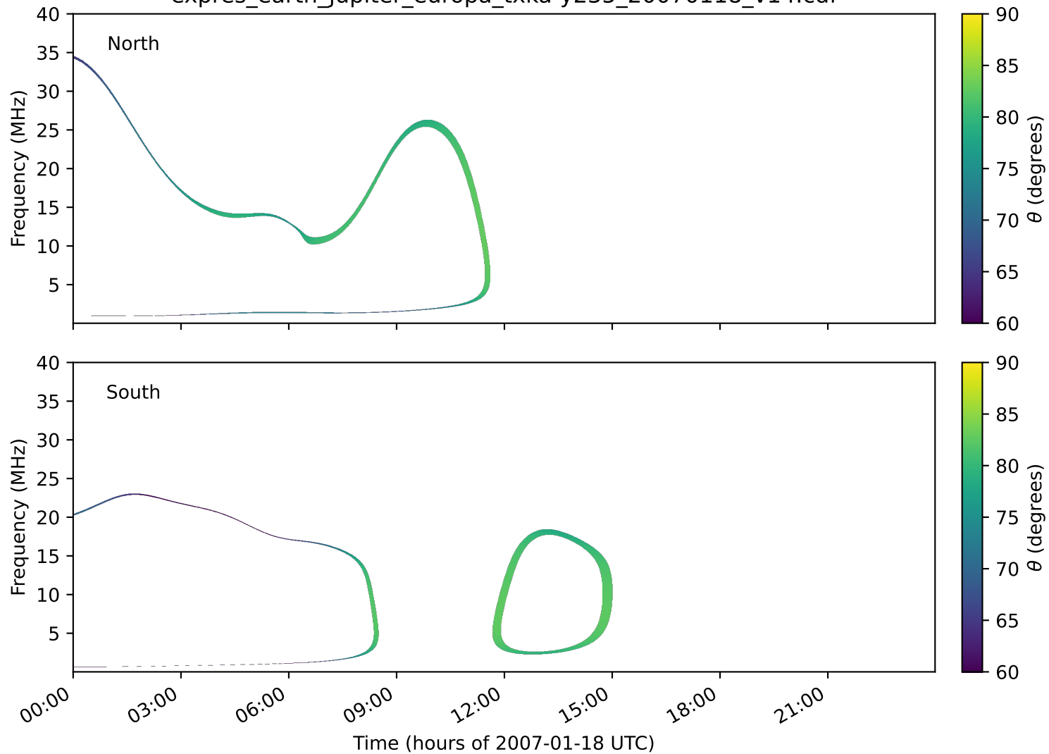
expres_earth_jupiter_europa_txka-y235_20070118_v14.cdf
