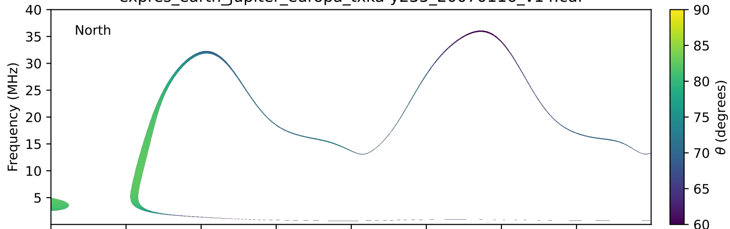
expres_earth_jupiter_europa_txka-y235_20070116_v14.cdf
