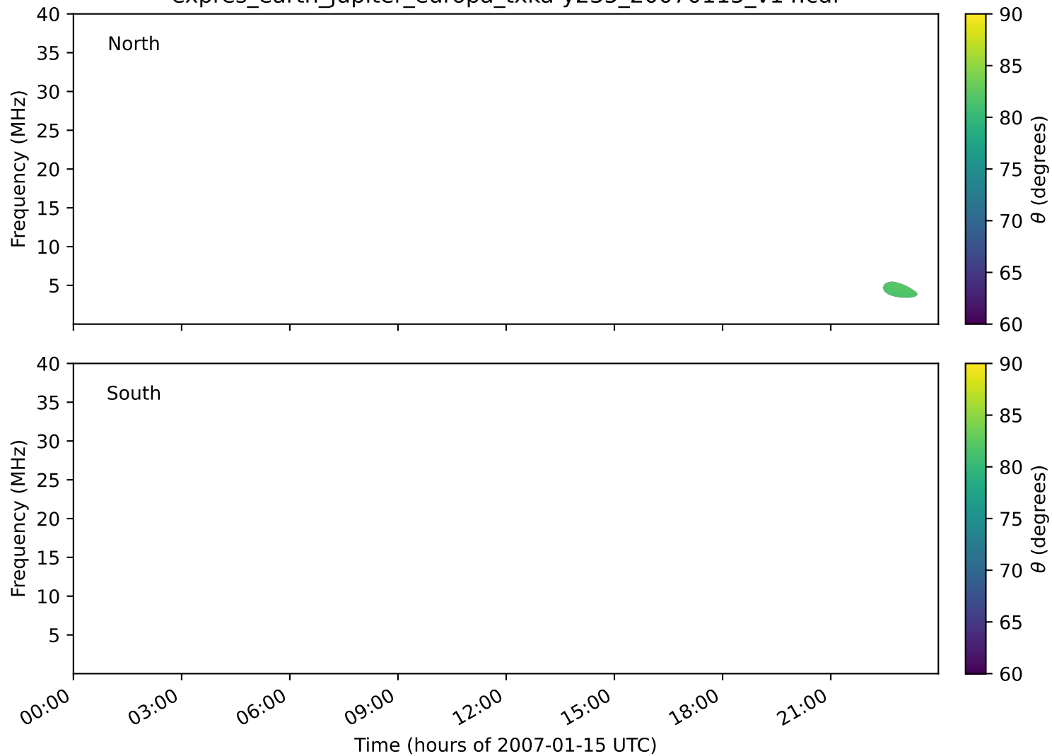
expres_earth_jupiter_europa_txka-y235_20070115_v14.cdf
