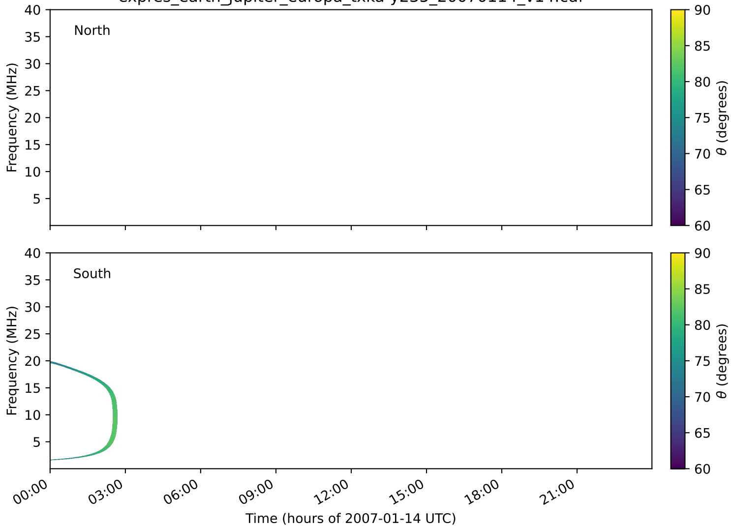
expres_earth_jupiter_europa_txka-y235_20070114_v14.cdf
