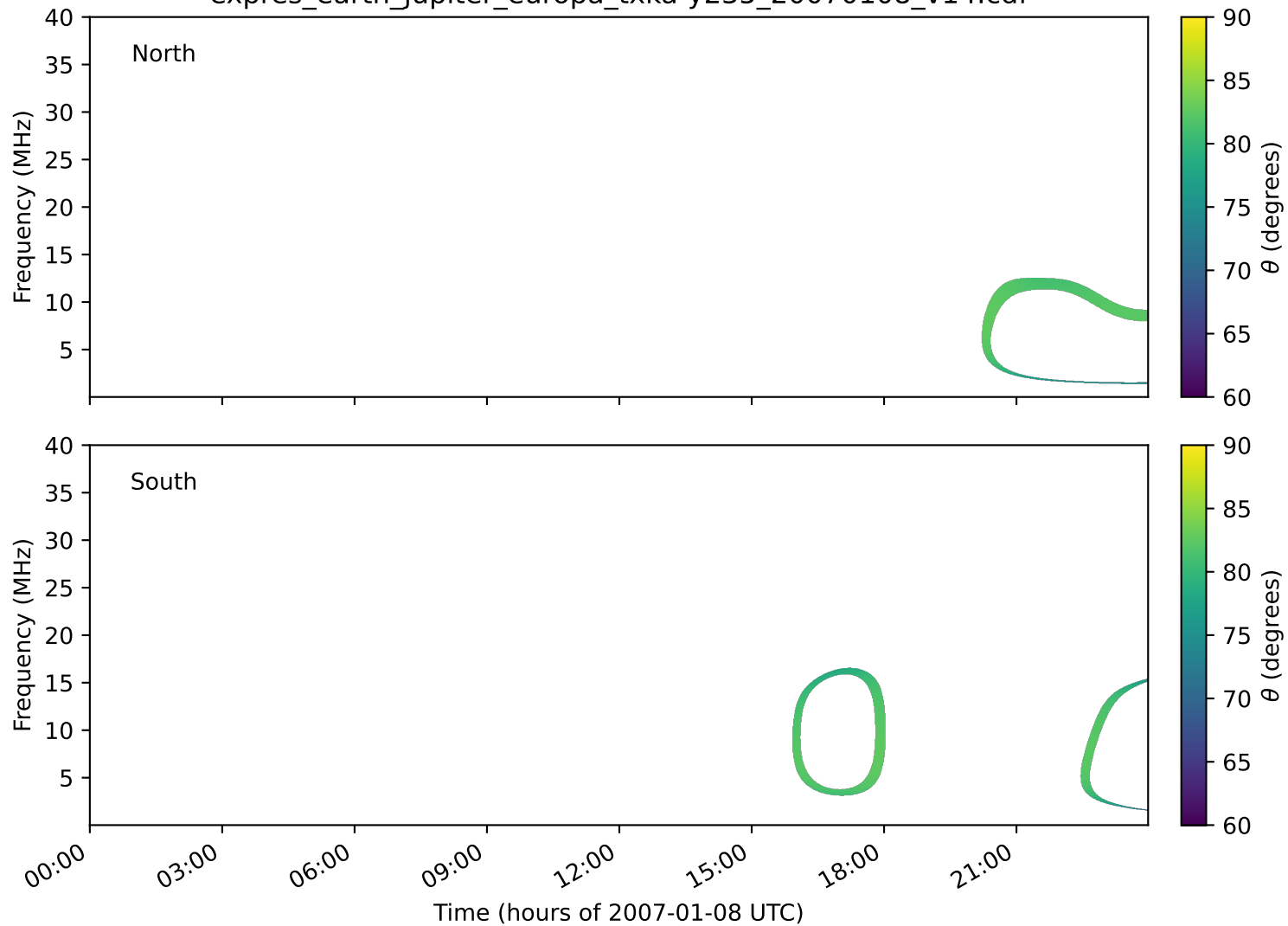
expres_earth_jupiter_europa_txka-y235_20070108_v14.cdf
