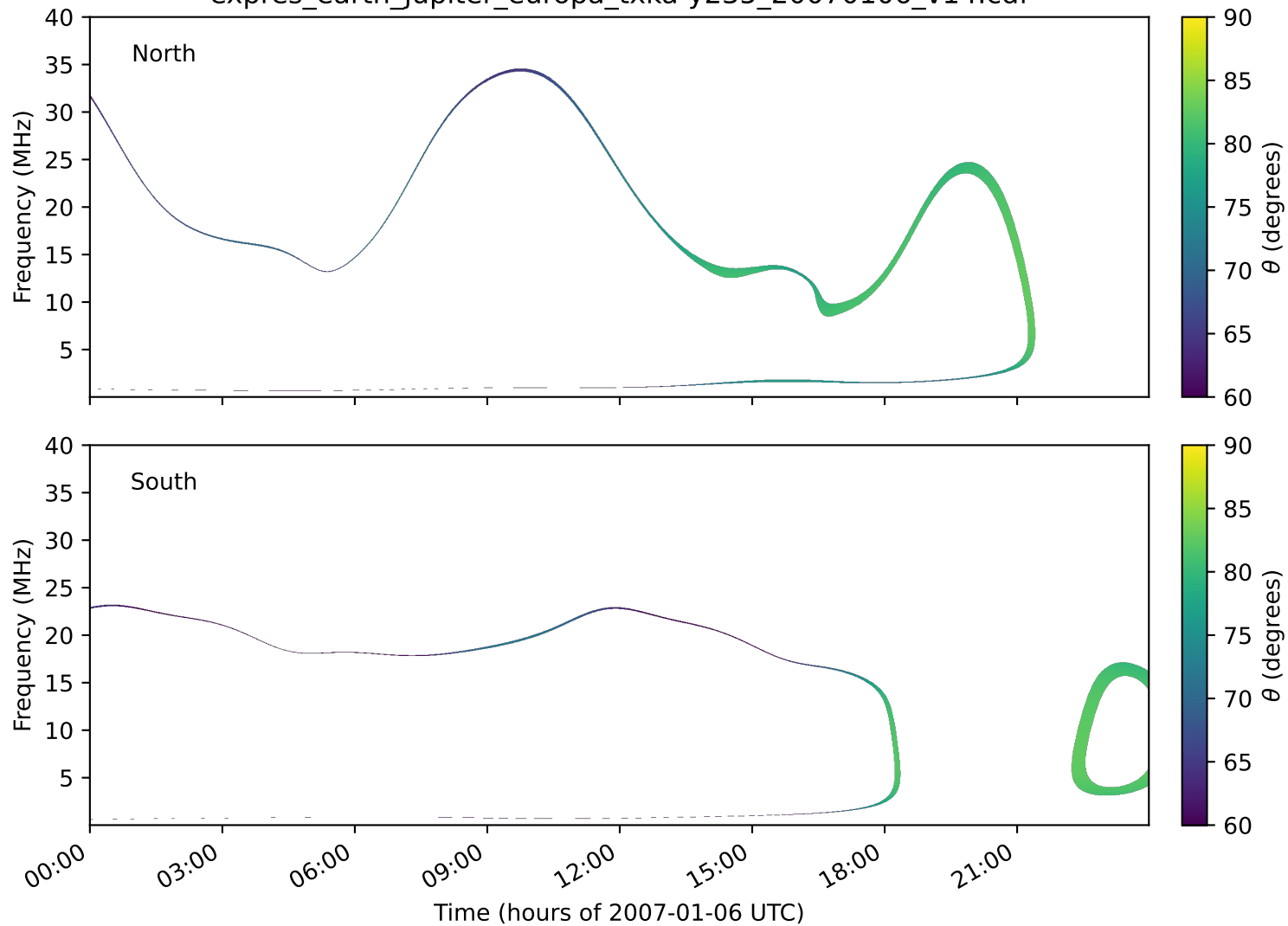
expres_earth_jupiter_europa_txka-y235_20070106_v14.cdf
