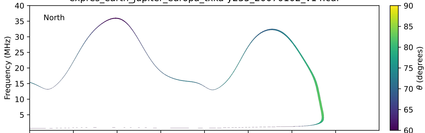
expres_earth_jupiter_europa_txka-y235_20070102_v14.cdf
