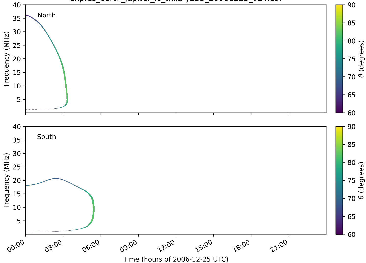
expres_earth_jupiter_io_txka-y235_20061225_v14.cdf
