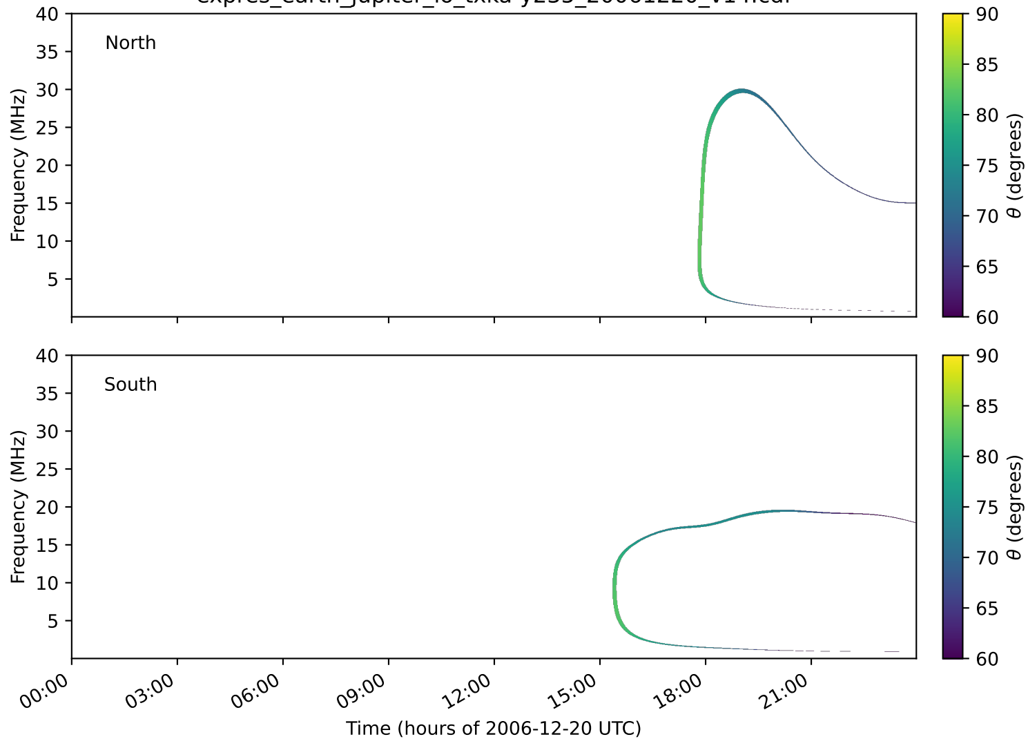
expres_earth_jupiter_io_txka-y235_20061220_v14.cdf
