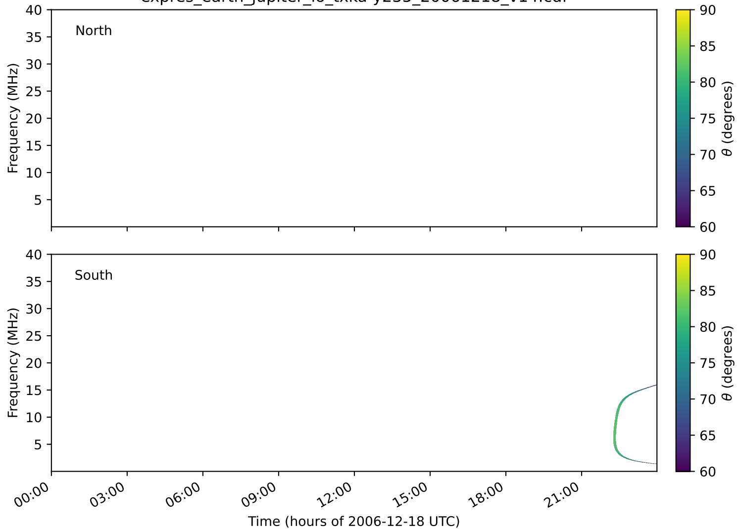
expres_earth_jupiter_io_txka-y235_20061218_v14.cdf
