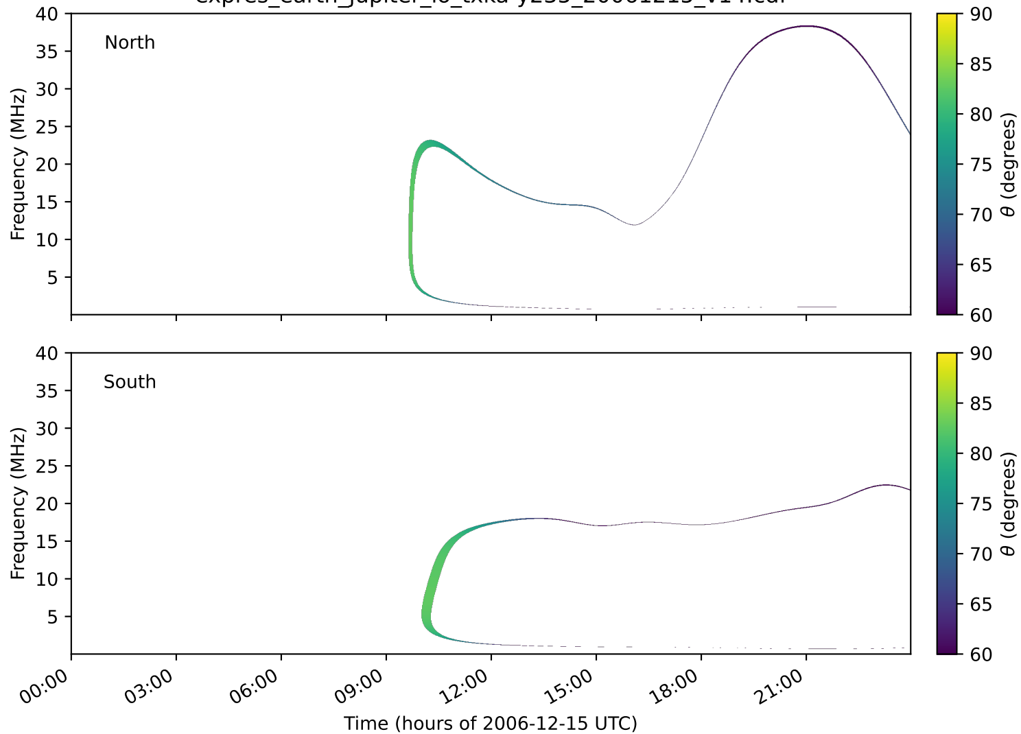
expres_earth_jupiter_io_txka-y235_20061215_v14.cdf
