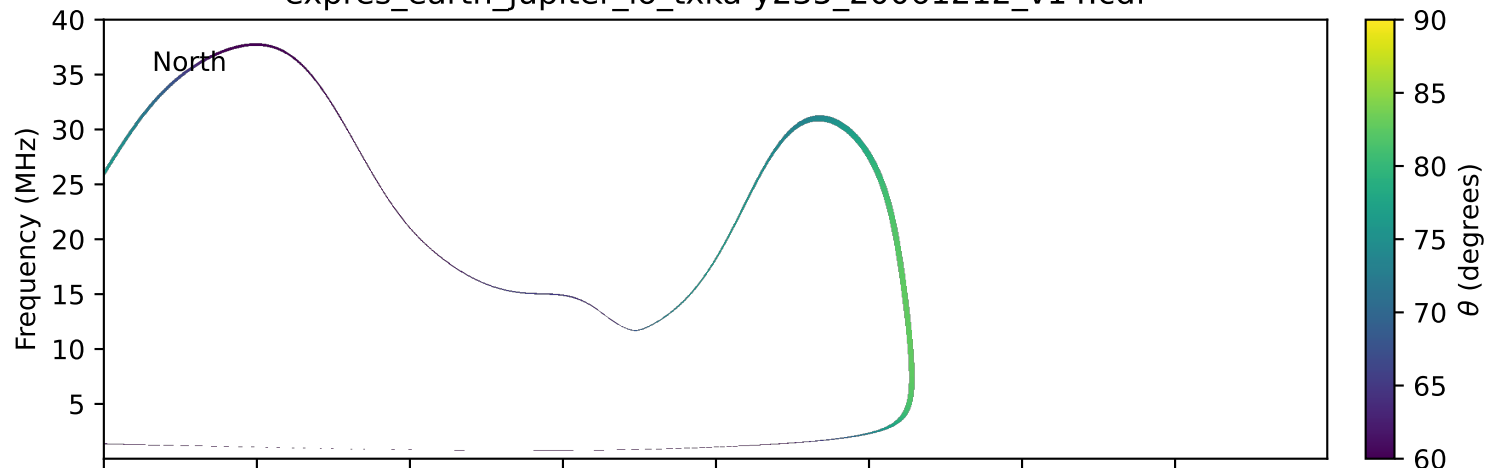
expres_earth_jupiter_io_txka-y235_20061212_v14.cdf
