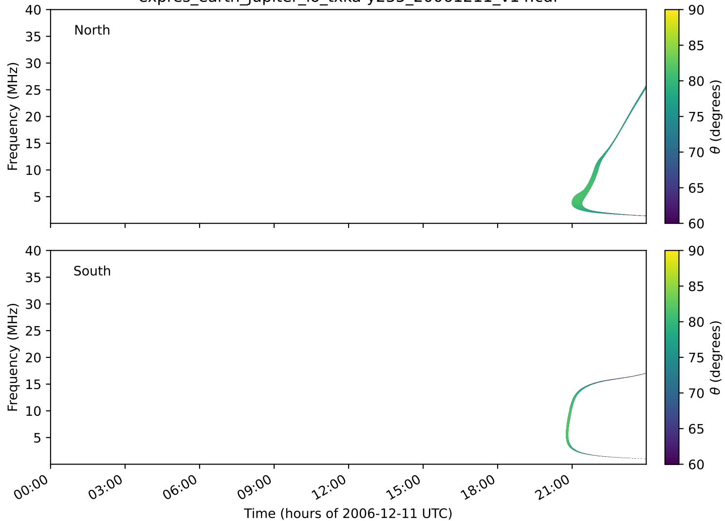
expres_earth_jupiter_io_txka-y235_20061211_v14.cdf
