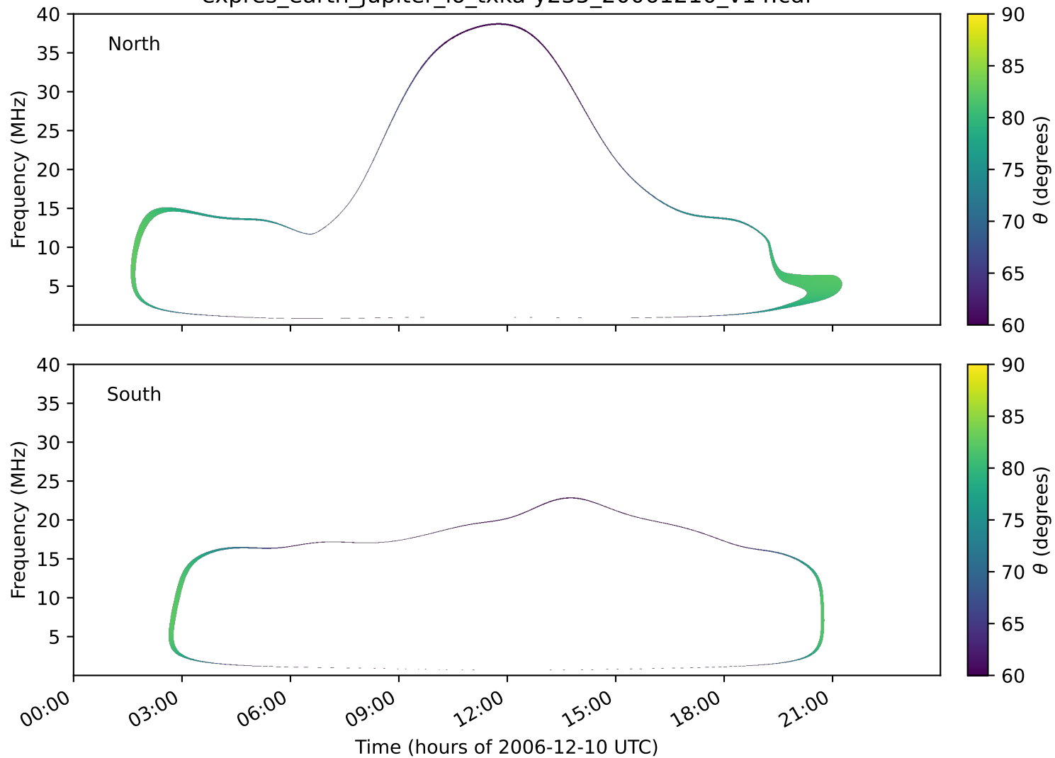
expres_earth_jupiter_io_txka-y235_20061210_v14.cdf
